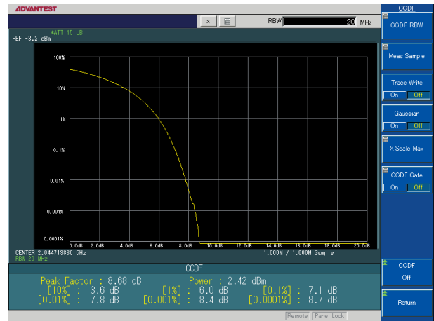
CCDF measurement results/3GPP (HSDPA) four carriers
