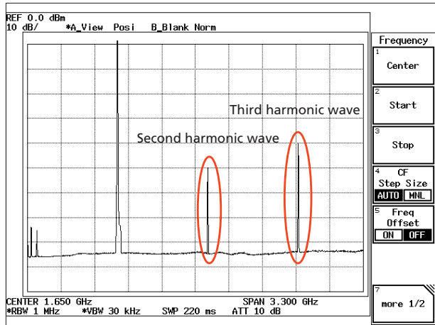
800 MHz input (previous instruments)
