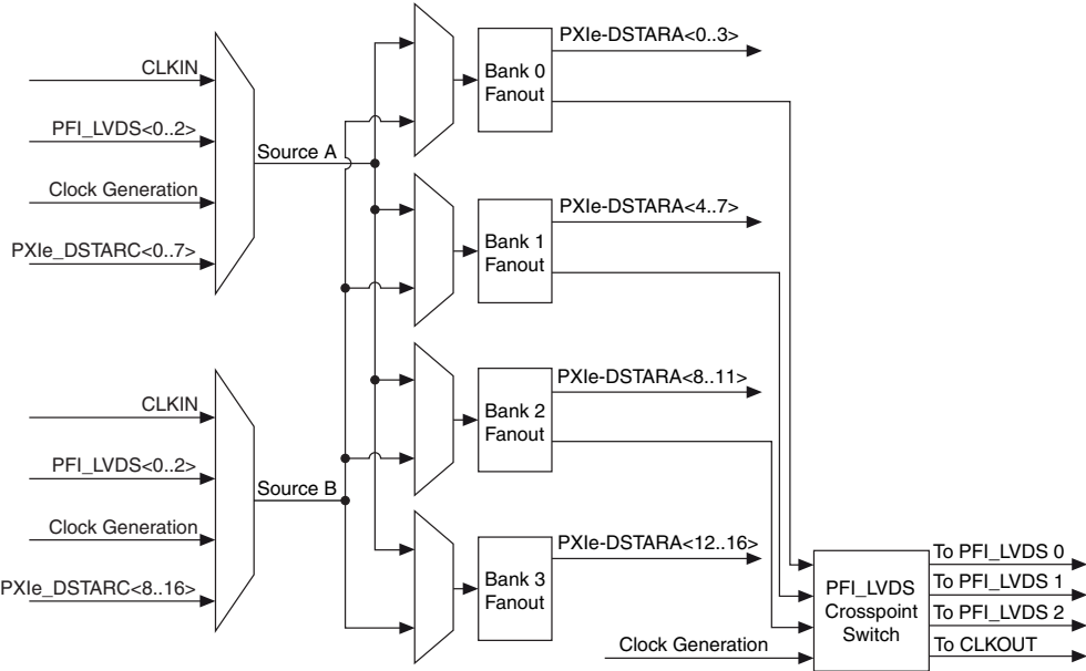
Figure 12. PXle-DStarA Topology
